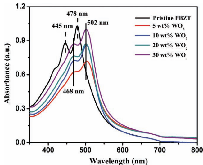
Figure 6. UV-Vis spectra of the pristine PBZT and \text{WO}_3/\text{PBZT} nanocomposite thin films after washing with DI water and drying in the vacuum oven overnight at 80 °C.
