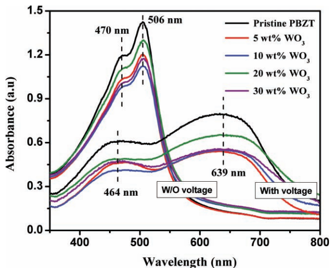
Figure 4. UV-Vis spectra of the pristine PBZT and \text{WO}_3/\text{PBZT} nanocomposite thin films with or without (W/O) applying voltage (3 V) during testing.
