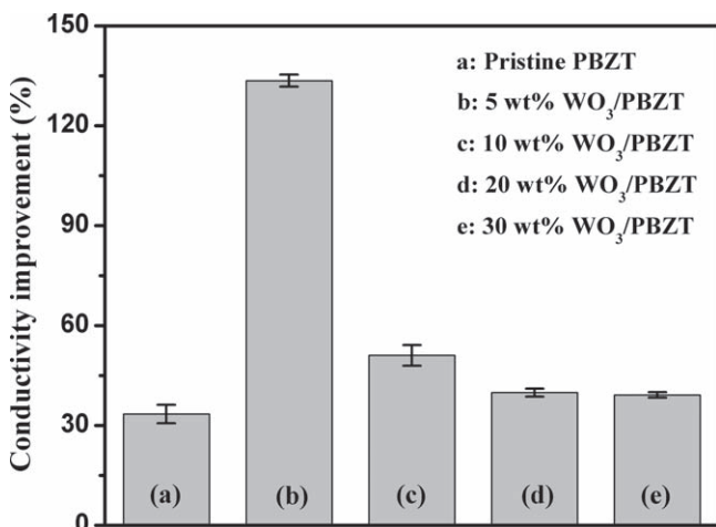
Figure 5. The electrical conductivity improvement for the PBZT/CSA and \text{WO}_3/\text{PBZT} nanocomposite thin films after applying 3 V potential.
